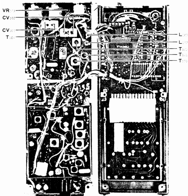
RECEIVER SECTION ALIGNMENT POINTS
