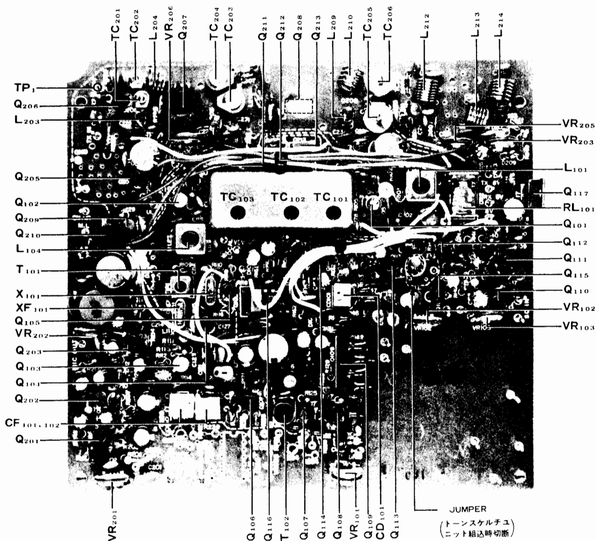
MAIN UNIT
