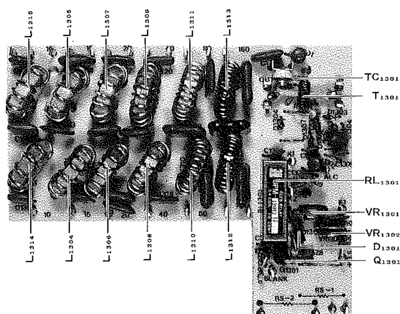
LPF UNIT (PB-1445B)
