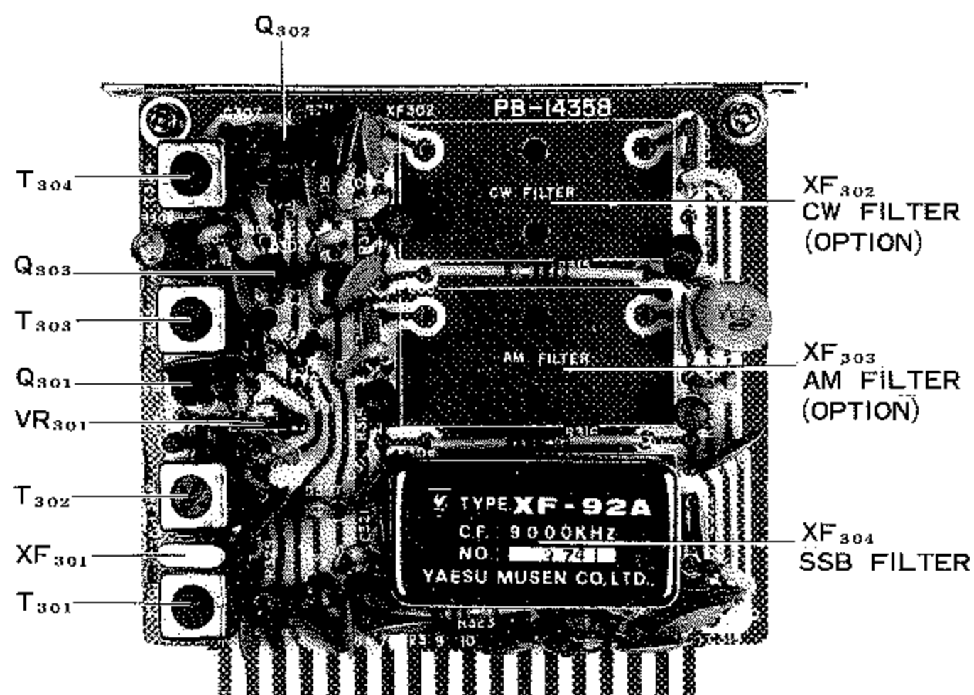
FILTER UNIT (PB-1435)
