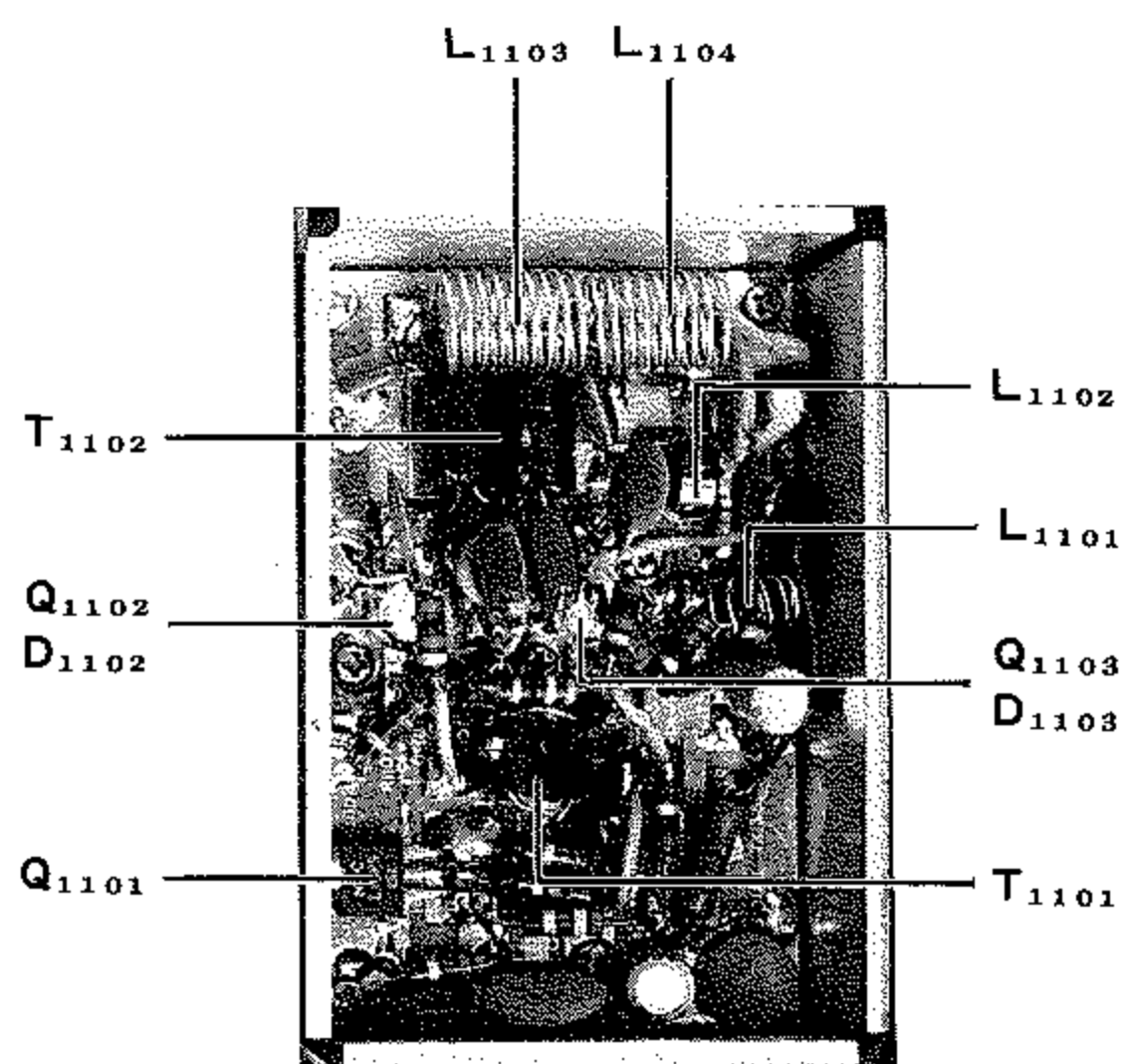
10W AMP UNIT (PB-1443)
