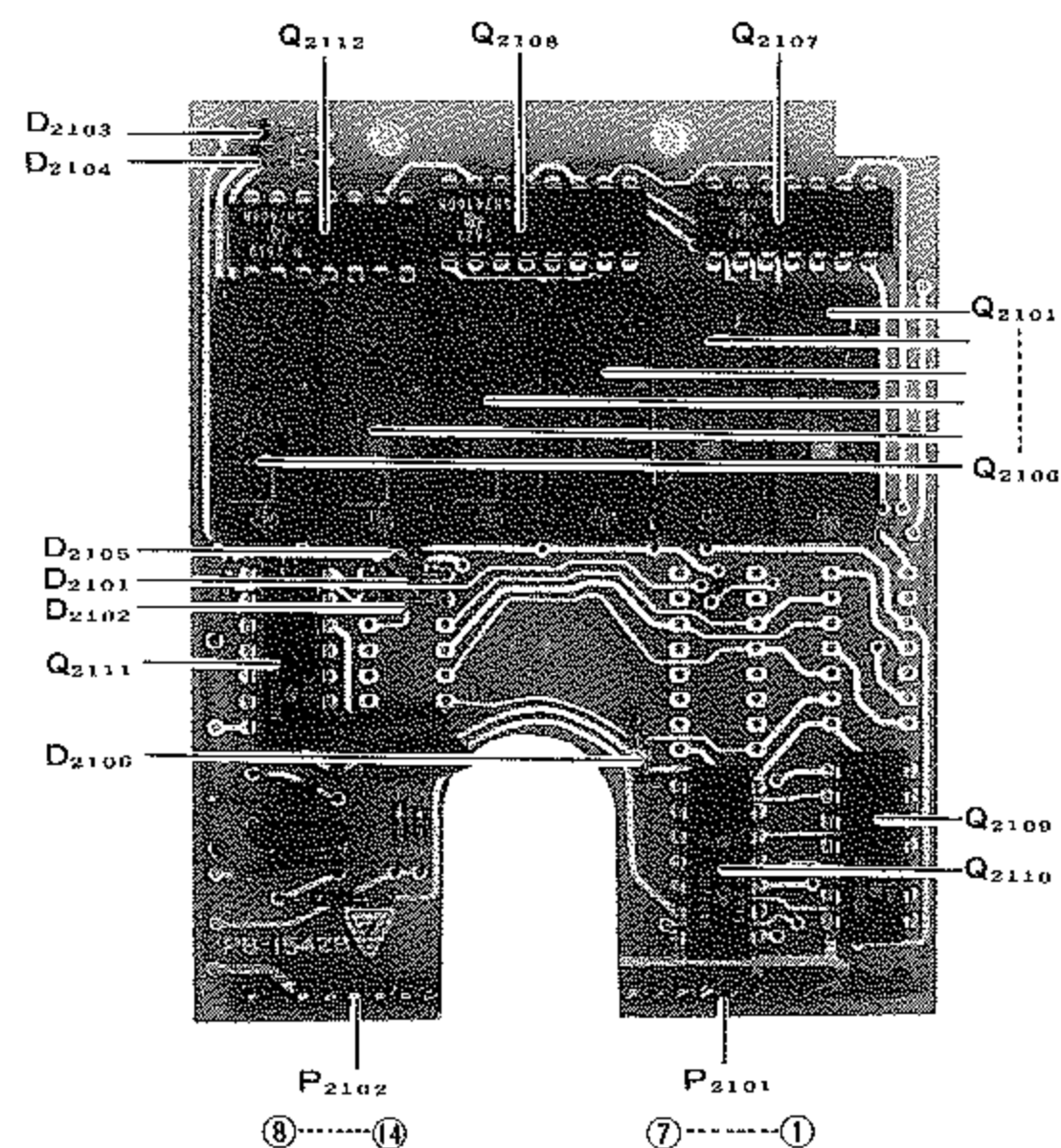
DISPLAY LOGIC UNIT (PB-1542B)
