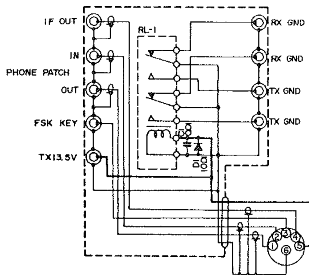
FT-301 RELAY BOX
