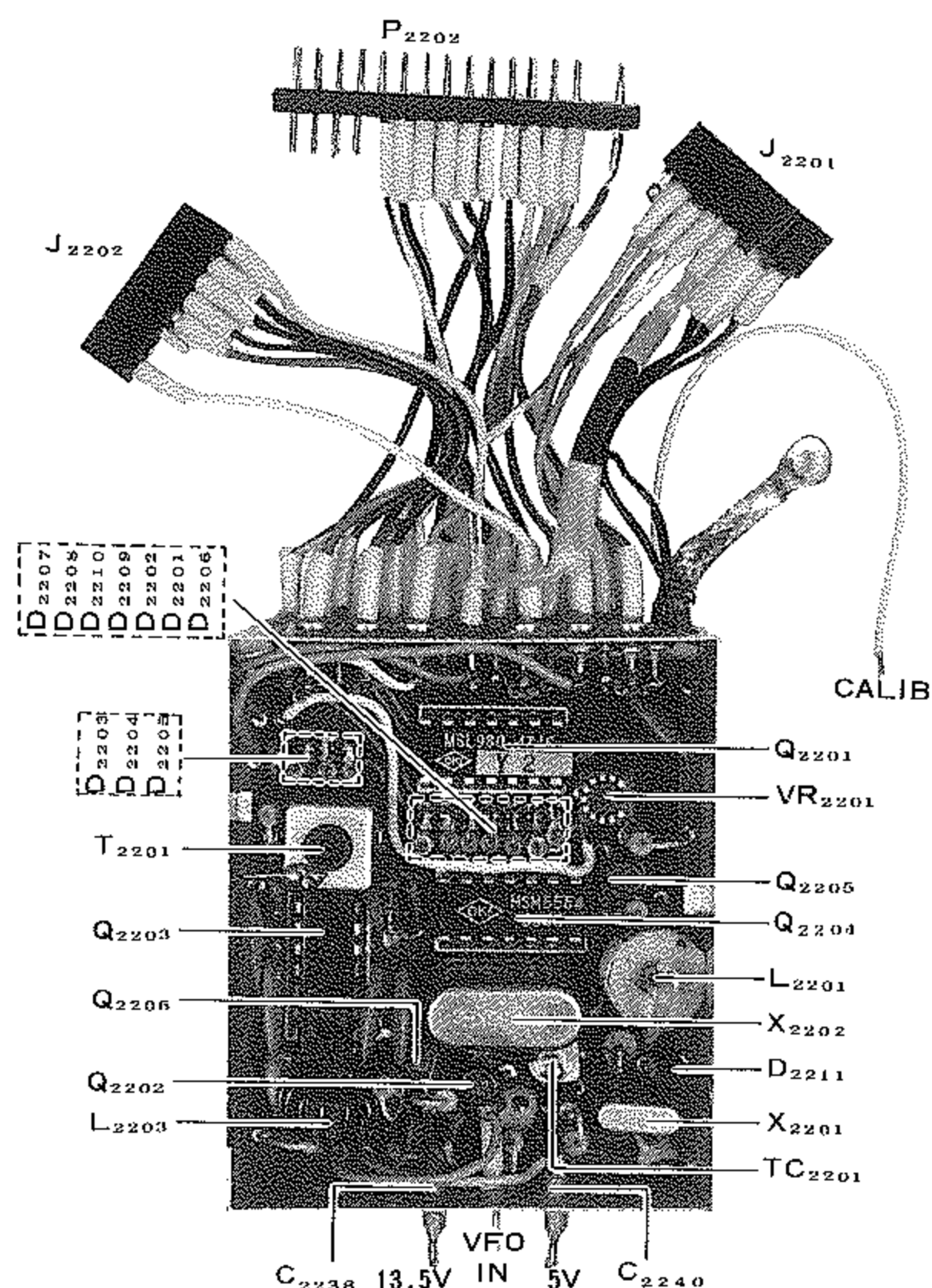
COUNTER MIXER UNIT (PB-1541D)
