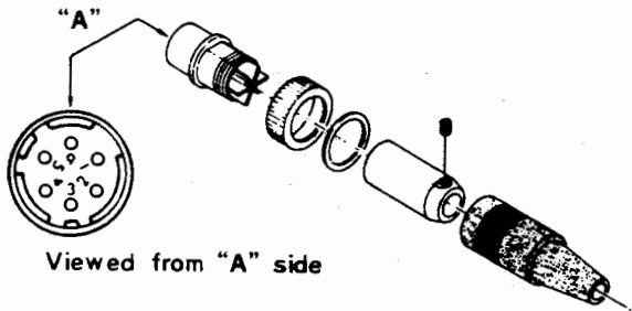
YM-24A Speaker/Microphone Connections
