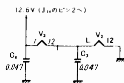
(A) FT-201
