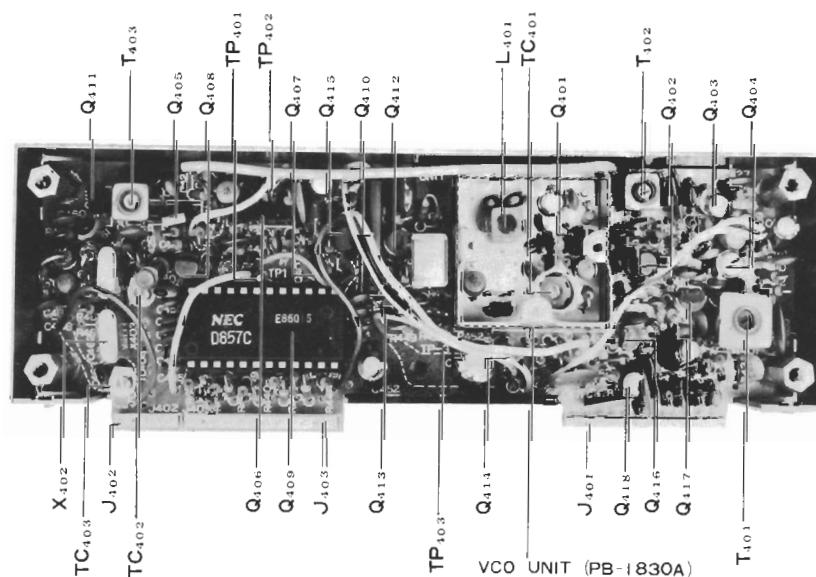
PLL UNIT (PB-I794)
