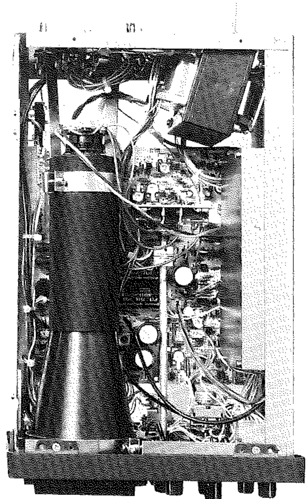
TOP VIEW
