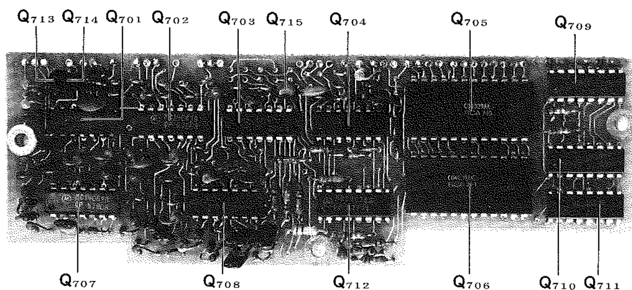
PLL CONTROL UNIT
