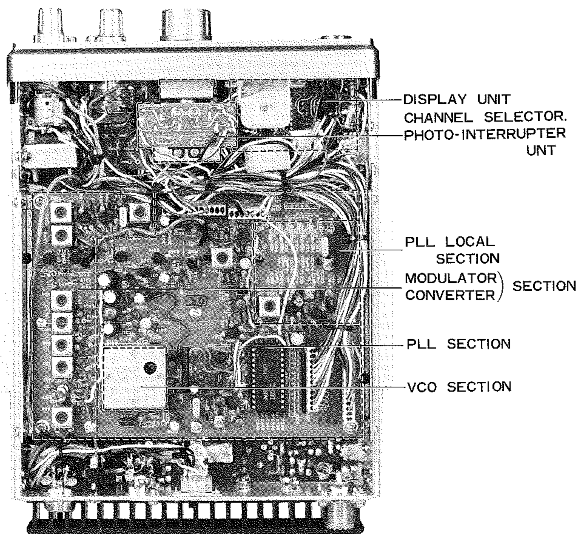
BOTTOM VIEW
