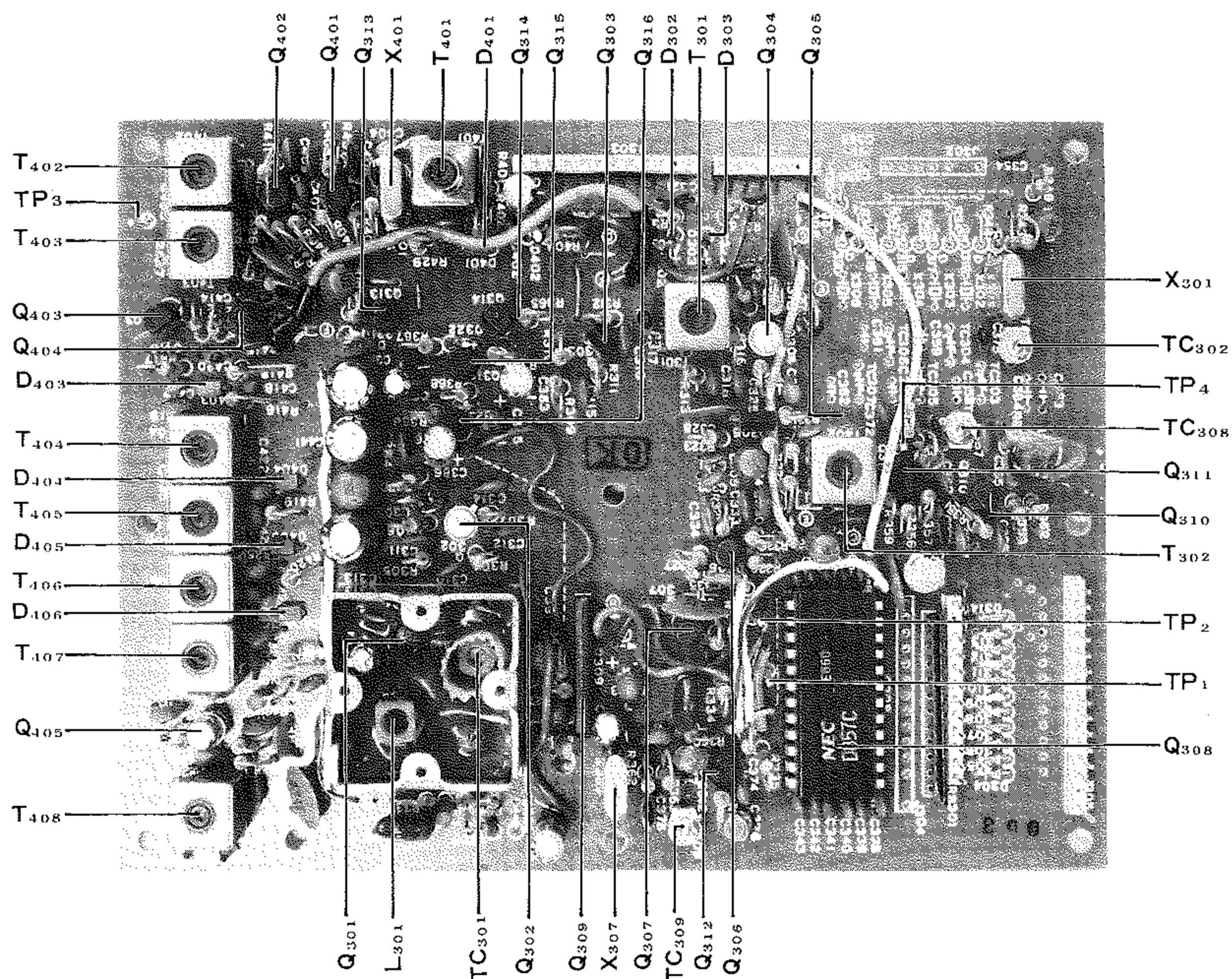
PLL UNIT
