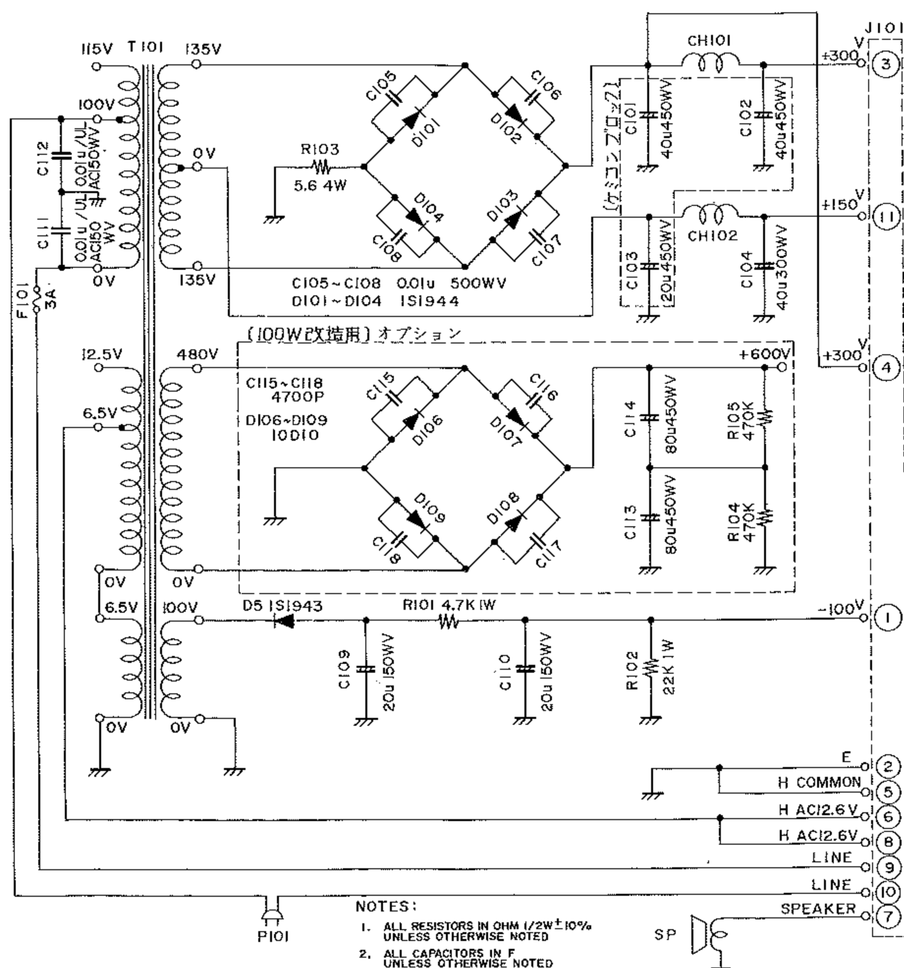
FP200S CIRCUIT DIAGRAM (FT200S 10W用 POWER SUPPLY)
