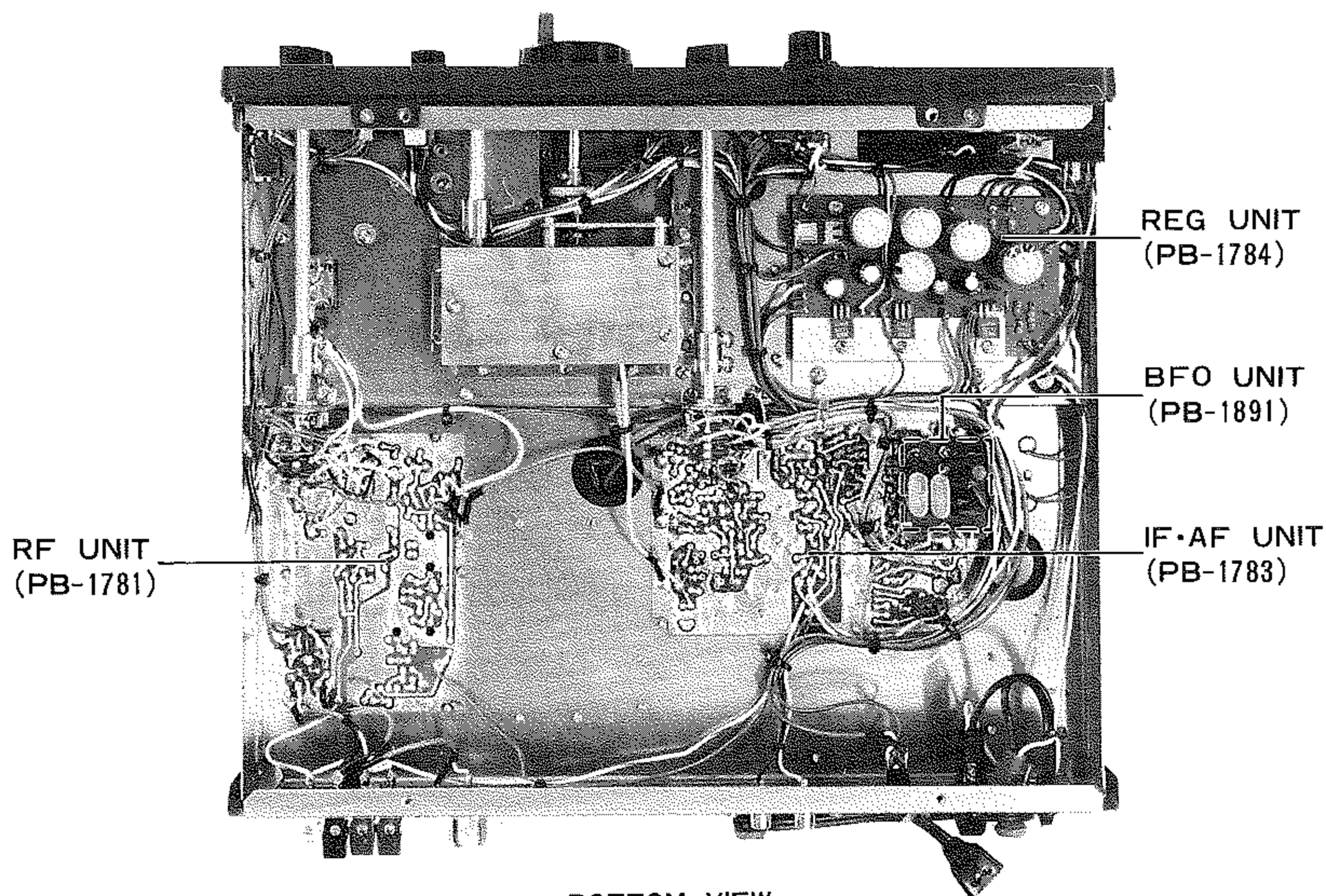
BOTTOM VIEW
