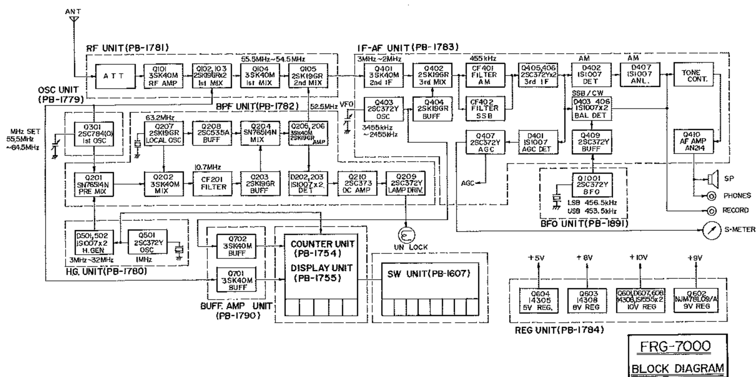
BLOCK DIAGRAM
