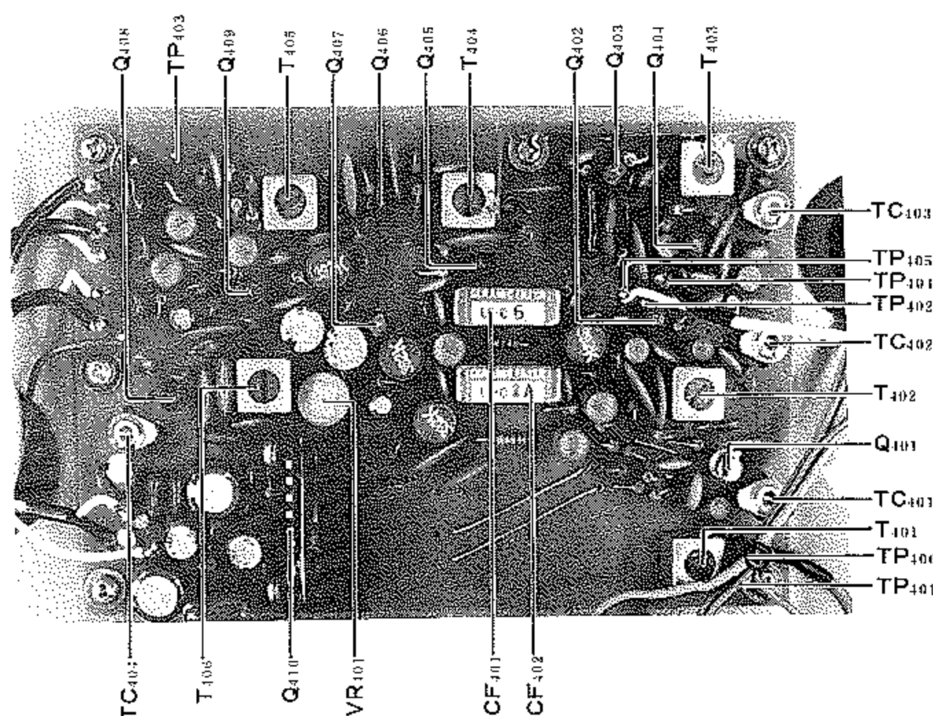
IF-AF UNIT (PB-1783)
