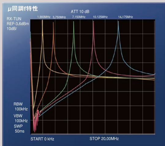
10 dB/Div・2 MHz/Div
