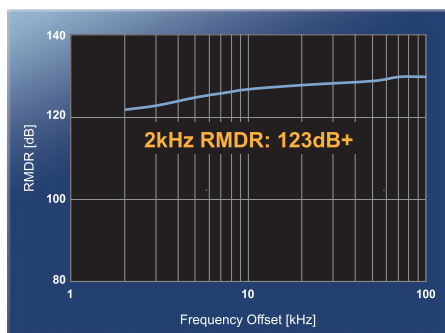
14MHz Band Reciprocal Mixing Dynamic Range (RMDR)
