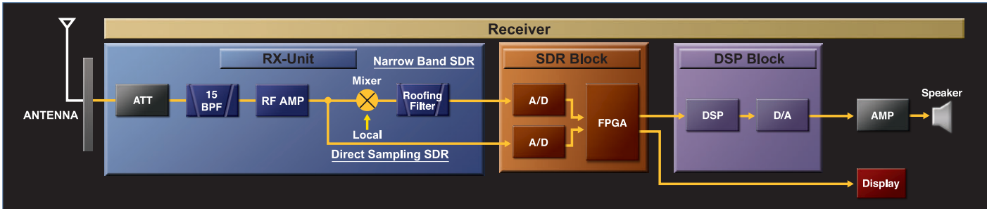
Receiver Block Diagram
